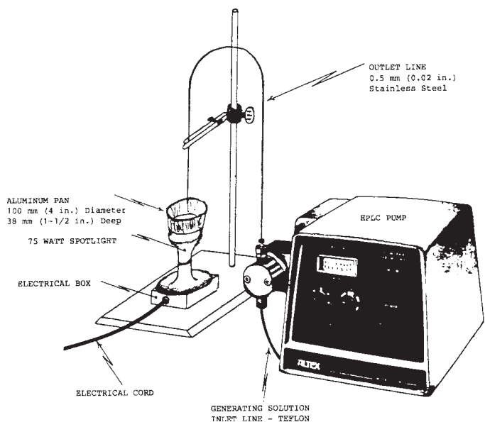
FIG. X2.1 Equipment Description
